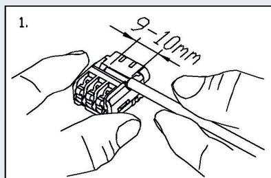
Gauge for stripping length
