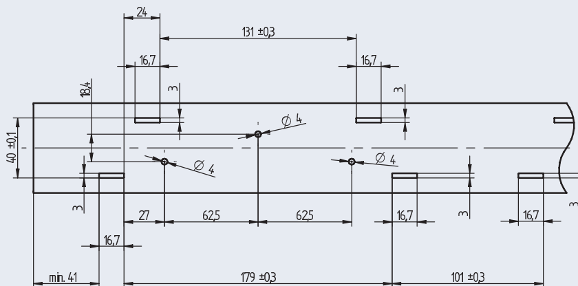
Cut-out metal sheet
